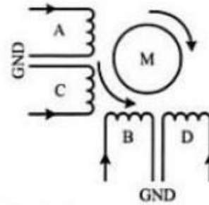
Fig. 2.18 2-Phase unipolar stepper motor
